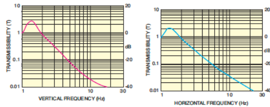
Vision IsoStation I-325 Series Isolators
